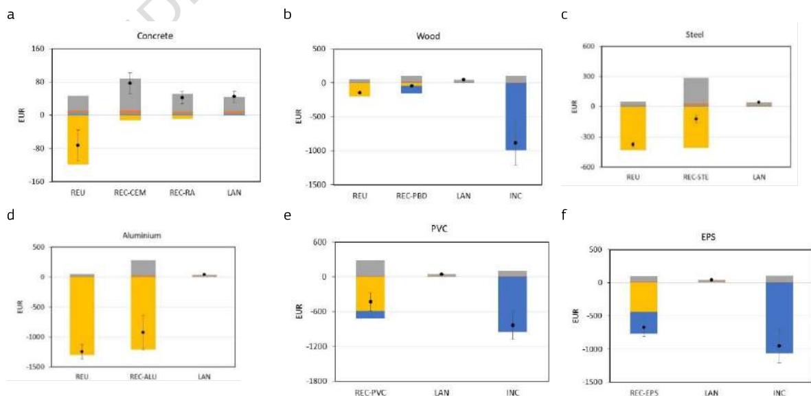
Figure 9. Environmental life cycle cost results per tonne of CDW fraction managed with breakdown of the contributions. Values above zero represent costs, while values below zero represent revenues. The final net impact, per each individual category, is the sum of costs and revenues and is represented with a black dot. The error bars represent the standard deviation around the net result. For the abbreviations used please refer to Table 11.
