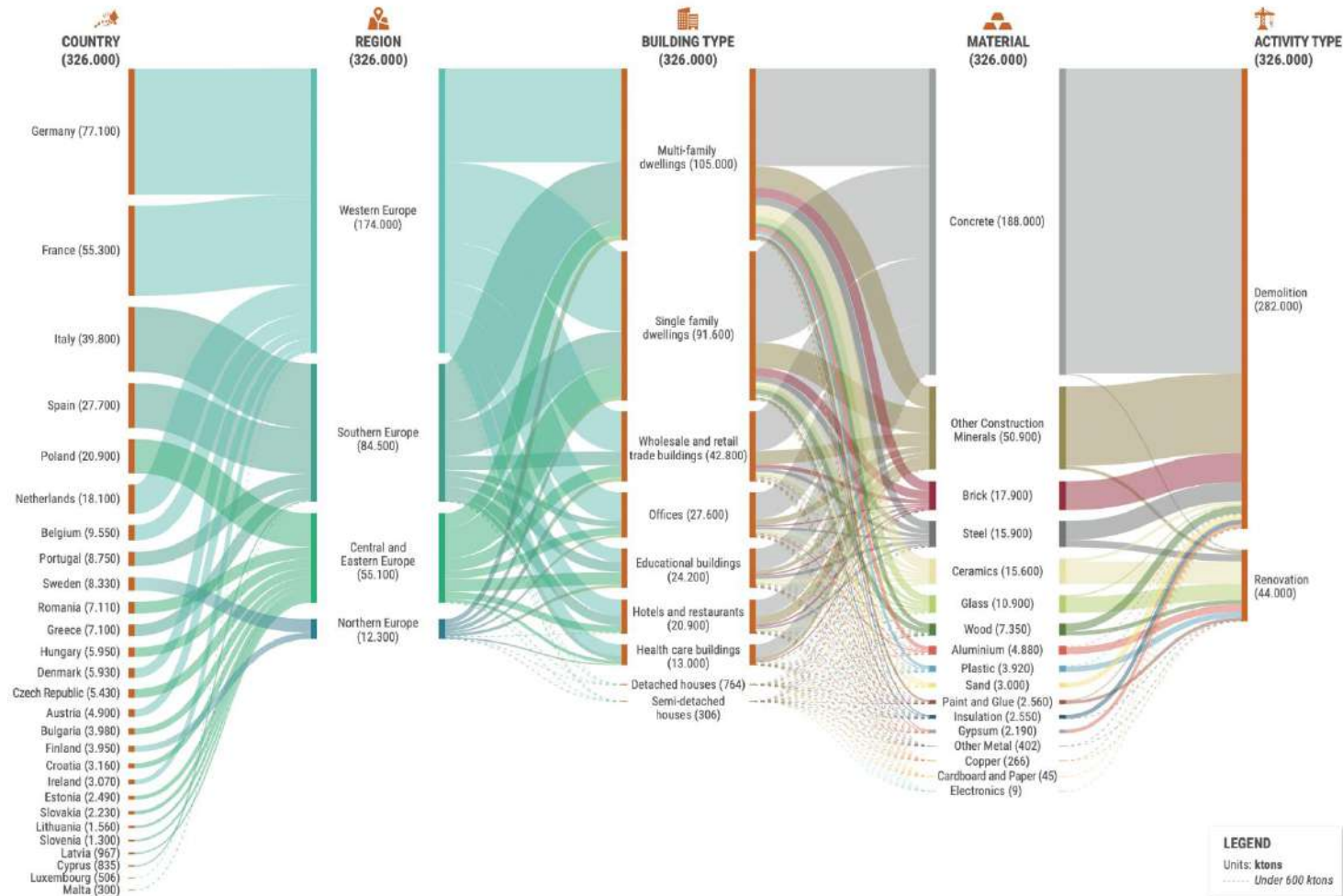
Figure 2. MFA showing origin of building-related material flows from countries, regions, building types and demolition and renovation activities in 2050 in the EU27 (infrastructure waste not included). Notice that the total inflow of material to construction and renovation was estimated to ca. 1 594 000 kt.
