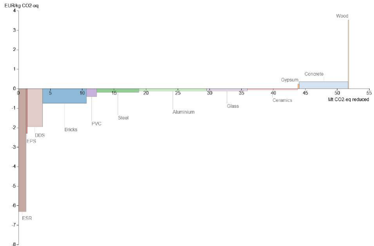
Figure 11. Marginal abatement cost curve for the maximum preparing for reuse potential (MPP) scenario. Notice that the impacts and costs of the baseline are accounted for as avoided. DDS: dredging spoils; EPS: expanded polystyrene; ESR: excavated soil; PVC: poly vinyl chloride.
