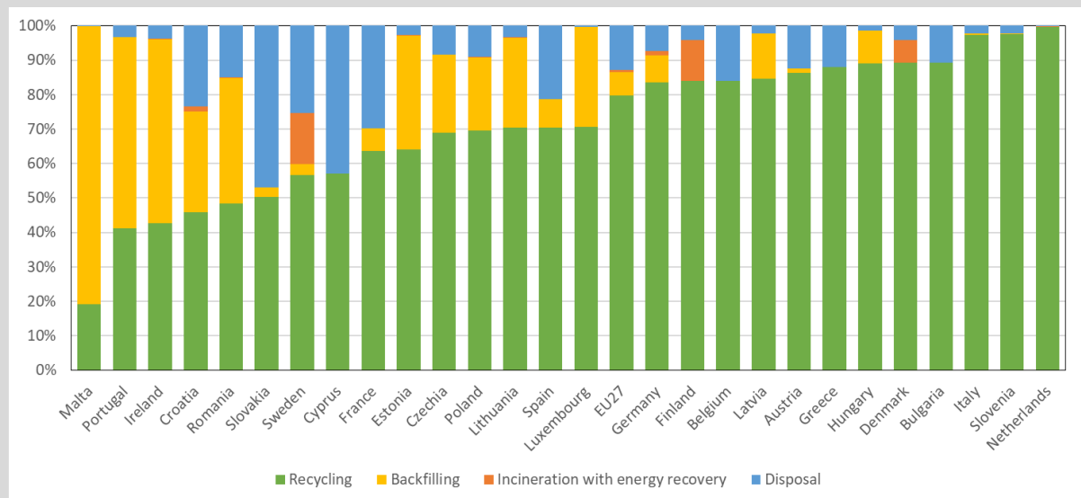
Figure B2. Treatment of the mineral fraction of CDW in the analysed Member States in 2016. Disposal is defined as landfill, incineration without energy recovery and other disposal.
