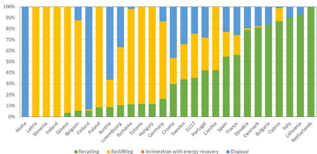
Figure 5. Treatment of the excavated soil fraction of CDW in the analysed Member States in 2020. Disposal is defined as landfill, incineration without energy recovery and other disposal. Note that data for Ireland 2020 is not available and data from 2018 has been used.
