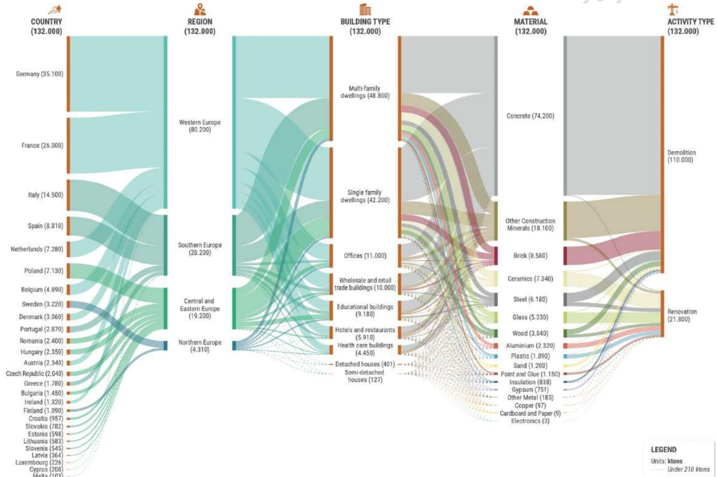
Figure 1. MFA showing the origin of building-related material flows from countries, regions, building types and demolition and renovation activities in 2020 in the EU27 (infrastructure waste not included). Notice that the total inflow of material to construction and renovation was estimated to ca. 1 004 000 kt.
