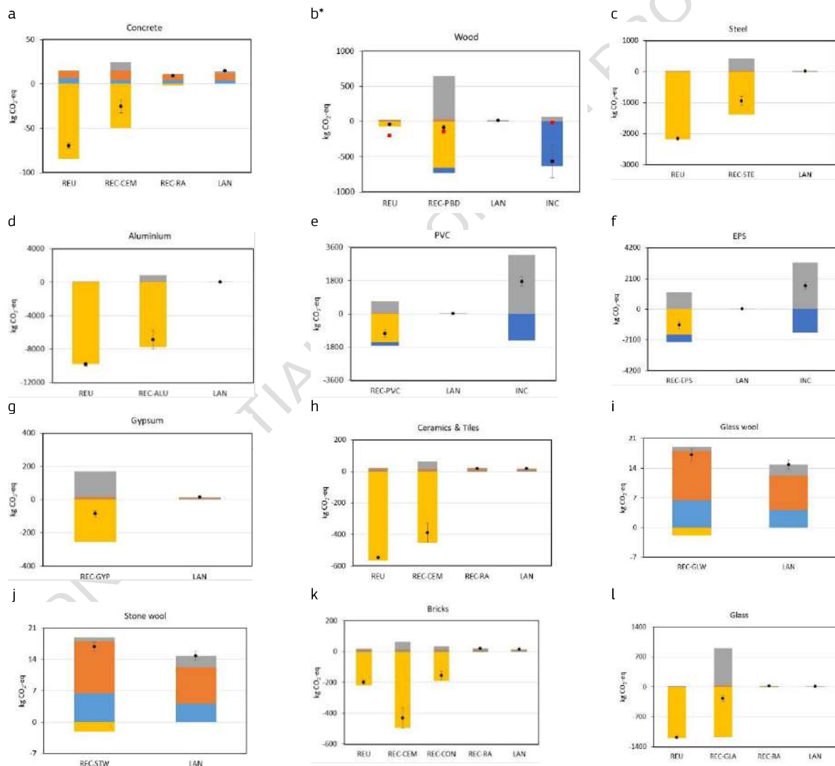
Figure 8. Characterised climate change results per tonne of CDW fraction managed with breakdown of the contributions in 2020. Values above zero represent burdens, while values below zero represent savings. The final net impact, per each individual category, is the sum of burdens and savings and is represented with a black dot. The error bars represent the standard deviation around the net result. For the abbreviations used please refer to Table 11.
